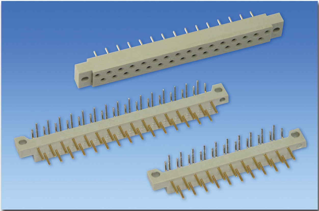
DIN 41617 PCB Connectors. Male and Female. 13, 21, and 31 contacts. Straight Solder Pin, Solder Tag, and Right Angle PCB Mount.
