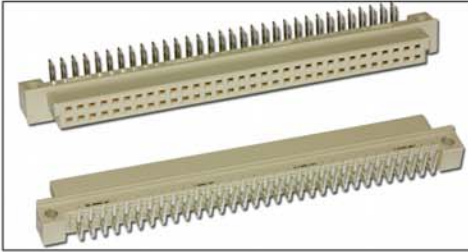
Type Q Female 64 Way RTA PCB Mount Row A + B Loaded : C2
