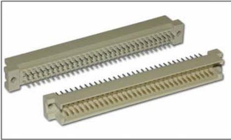
Type R Male 64 Way ST Solder Pin Row A + C Loaded : C2
