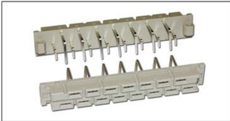
H15 Female (Reversed) RTA PCB Mount 15 Amp Class 1
