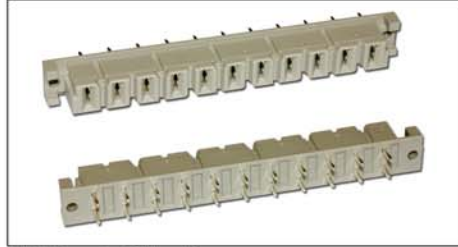
H11 Female Solder Pin 20 Amp Class 1
