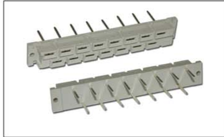
H15 Female 13mm Solder Pin 15 Amp Class 1
