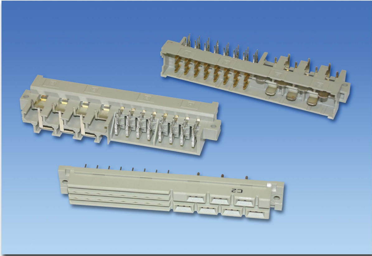
DIN 41612 Type F24+H7 Mixed Contact Connectors. Male Right Angle PCB Mount and Female Slimline Straight Pin PCB Mount. 24 Signal Contacts Type F and 7 Power Contacts Type H.
